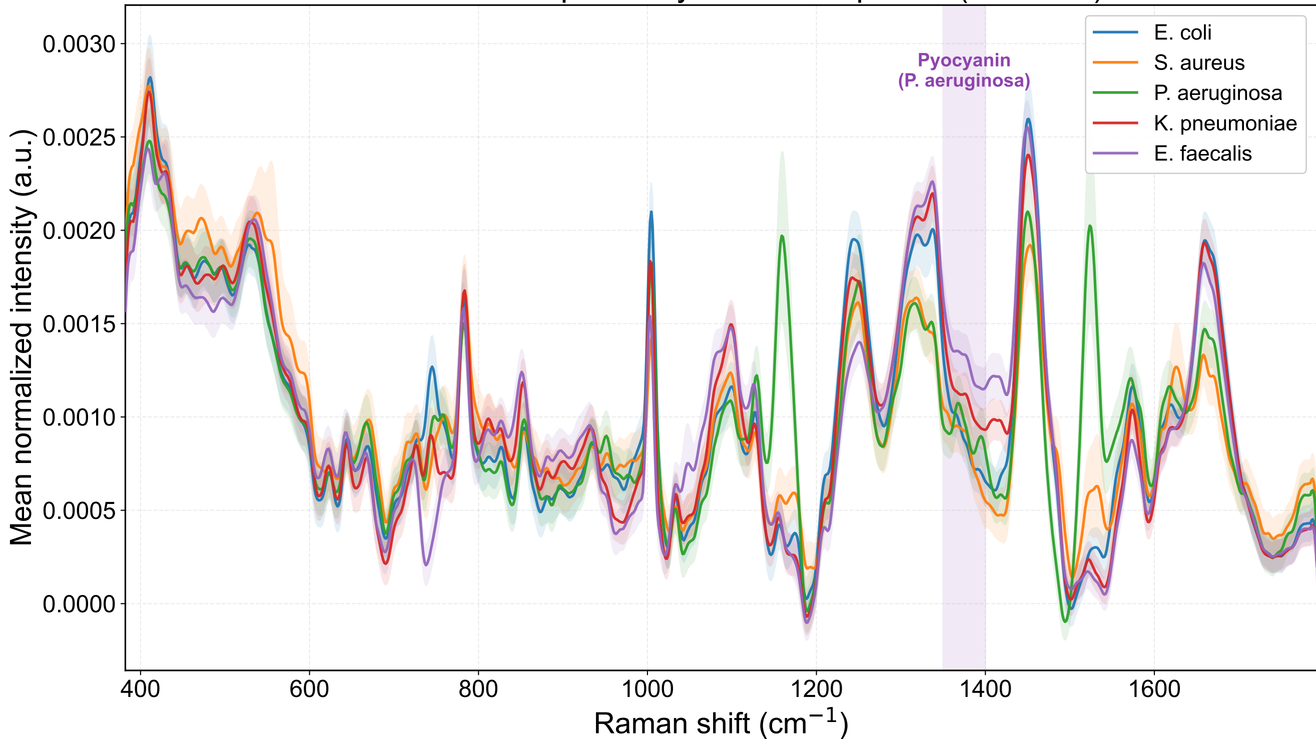
Mean Raman Spectra by Bacterial Species ( \pm 0.5 SD)
